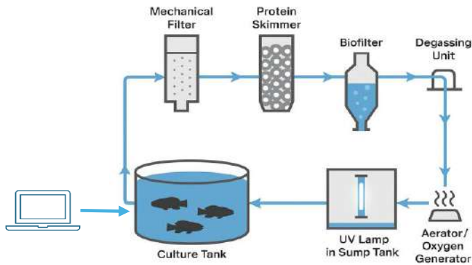
Fig 38: Recirculating Aquaculture System (RAS) for Grouper Farming
